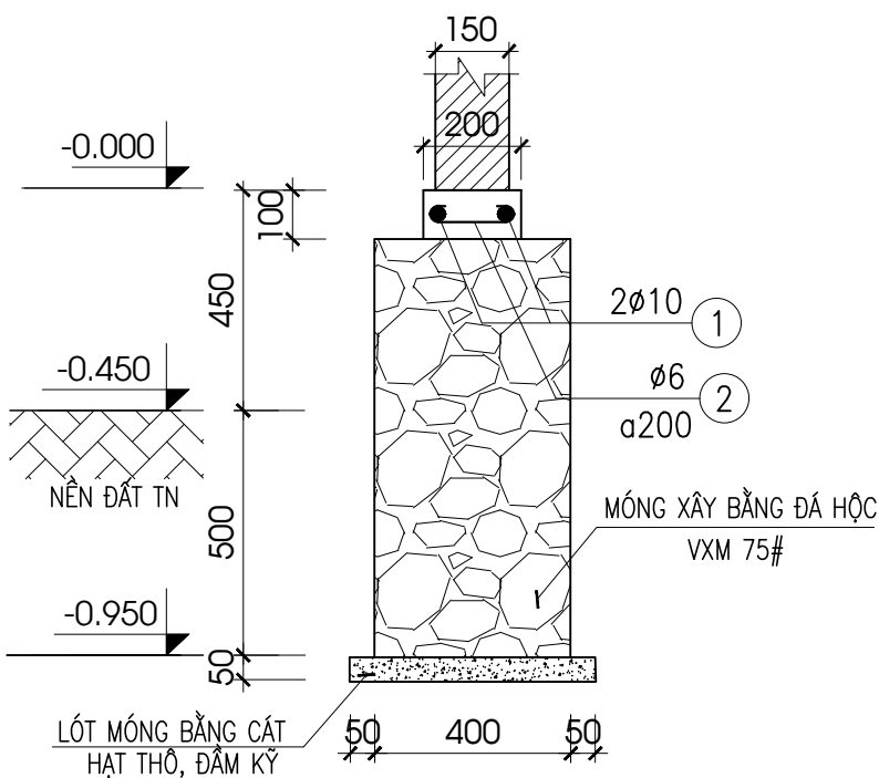
MÓNG MT1 (SL: 01; L = 22.100)
